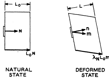
FIG. 1. Change of propagation direction \mathbf{n} and path length L with change of static deformation. (The propagation direction remains perpendicular to the reflecting faces of the specimen while the material line segment L_0\mathbf{N} is rotated and stretched into \lambda_N L_0\mathbf{m} . The perpendicular distance between the faces changes from L_0 to L = \lambda_N L_0 \mathbf{m} \cdot \mathbf{n} .)
